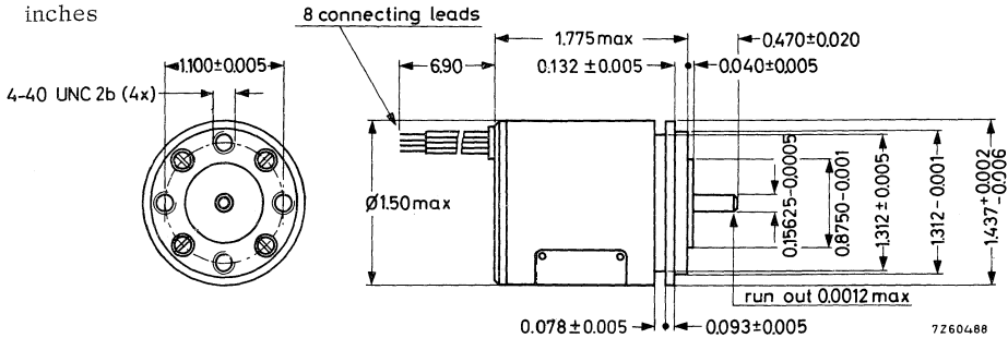
Fig. 1b. SMD11 in inches
