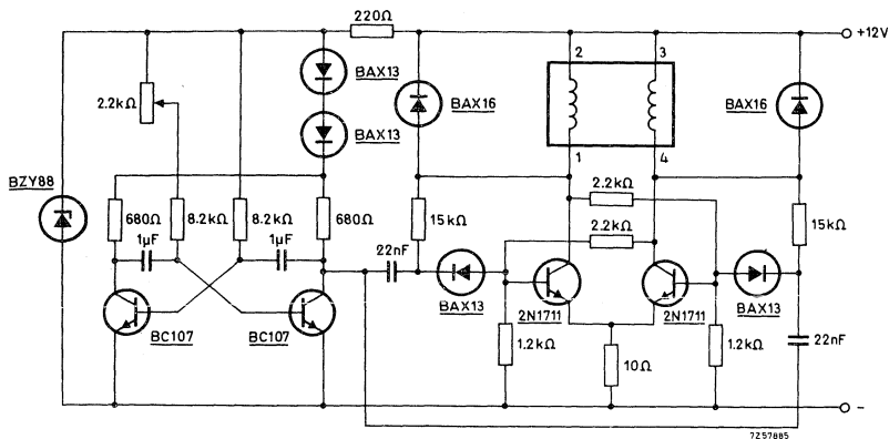
Circuit diagram of inverter 9904 131 03001, for use in conjunction with unidirectional motors.
