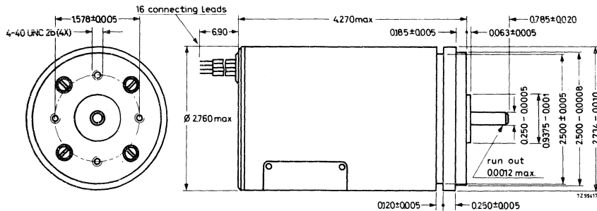
Fig. 1b. SMD 21 (in inches)
