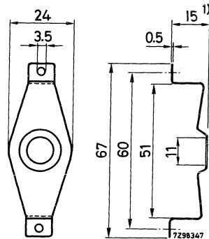
Bracket 9904 131 01003
