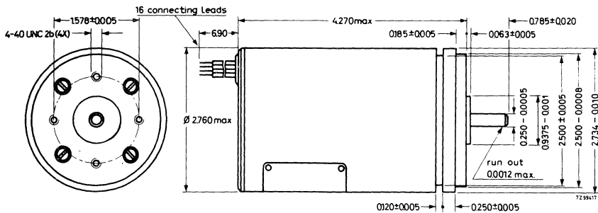
Fig. 1b. SMD 25 (in inches)
