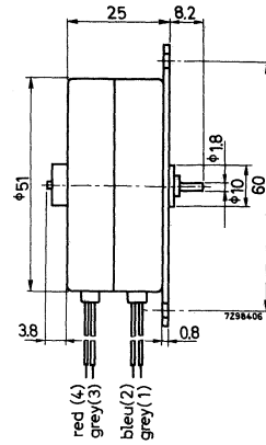
Reversible motor 9904 111 04611
