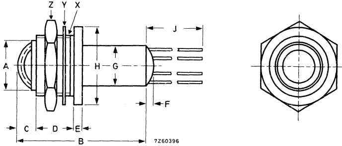
Model K21702-M2, Rear panel mounting
