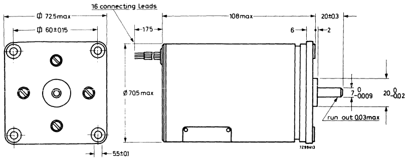
Fig. 1a. PD 20 (in mm)
