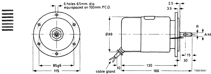
Fig. 1. Spigot-flange types of d. c. tachogenerators.
