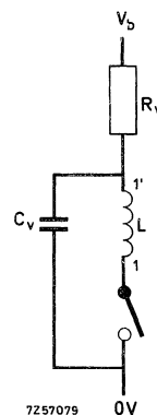
Fig. 3. Connection of the compensating network R_V - C_V . ( L is the stator phase winding 1; the numbers 1 and 1' refer to the leads to and from phase 1. The switch can be a transistor, as in the electronic switches, described below).
