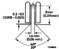
Detailed view of the slot
