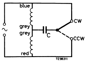
Coils in series
