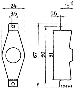
Bracket 9904 131 01001
