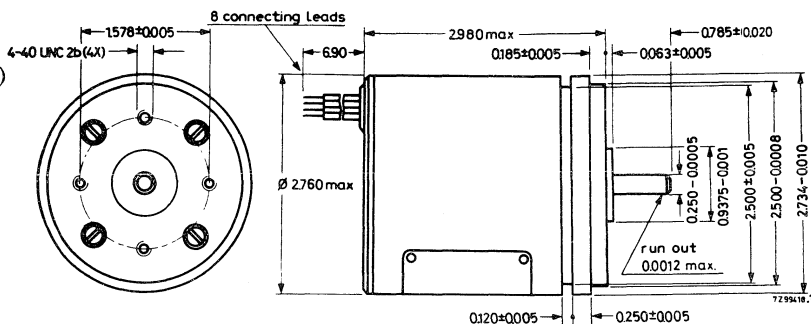
Fig. 1b. SMD 23 (in inches)
