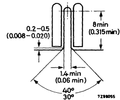
Detailed view of the slot
