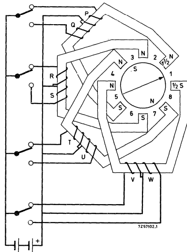
Fig. 2. Diagrammatic representation of an 8-phase, 2-pole motor: rotor at position 1.
