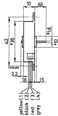
Unidirectional motor 9904 110 05806 or 9904 110 05808
